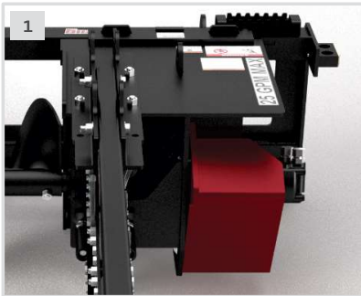
1. 4-POSITION DEPTH ADJUSTMENT SYSTEM ALLOWS OPERATOR TO SET DESIRED TRENCHING DEPTH
