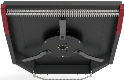
DETAIL UNDER DECK
