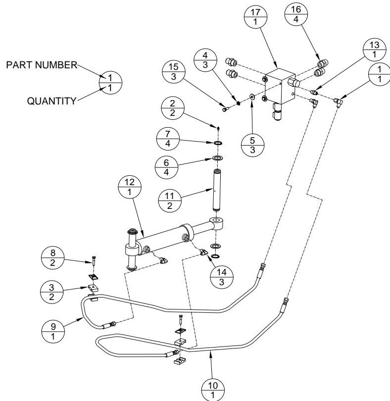
Standard Hydraulic Angle Connections
