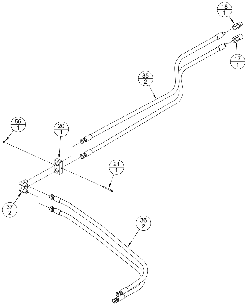
Standard Coupler Assembly
